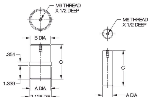
Center Pin
